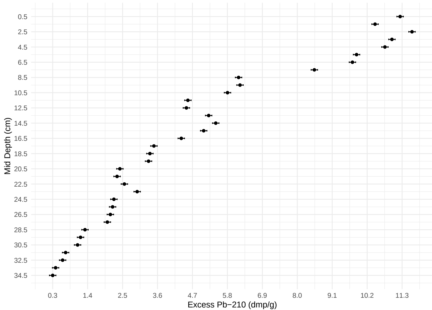
Excess Pb-210 vs Depth
